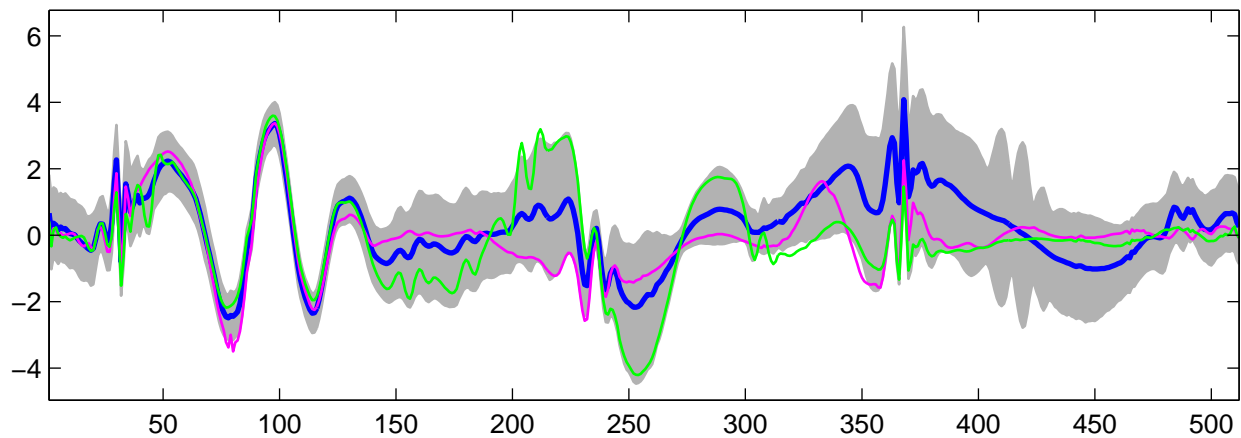
Estimated U_{11}(t) using G-WFMM: t_1 data, run 4
