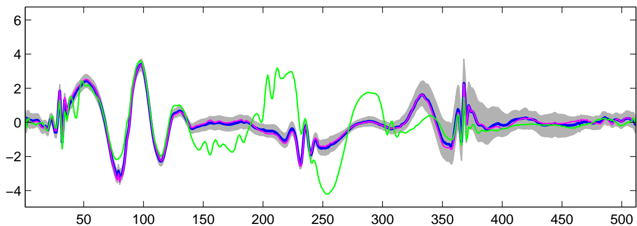
Estimated U_{11}(t) using R-WFMM: t_1 data, run 4
