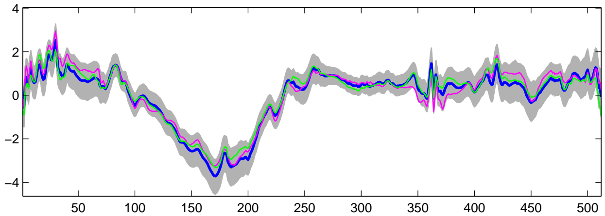
Estimated U_{12}(t) using R-WFMM: DE data, run 4
