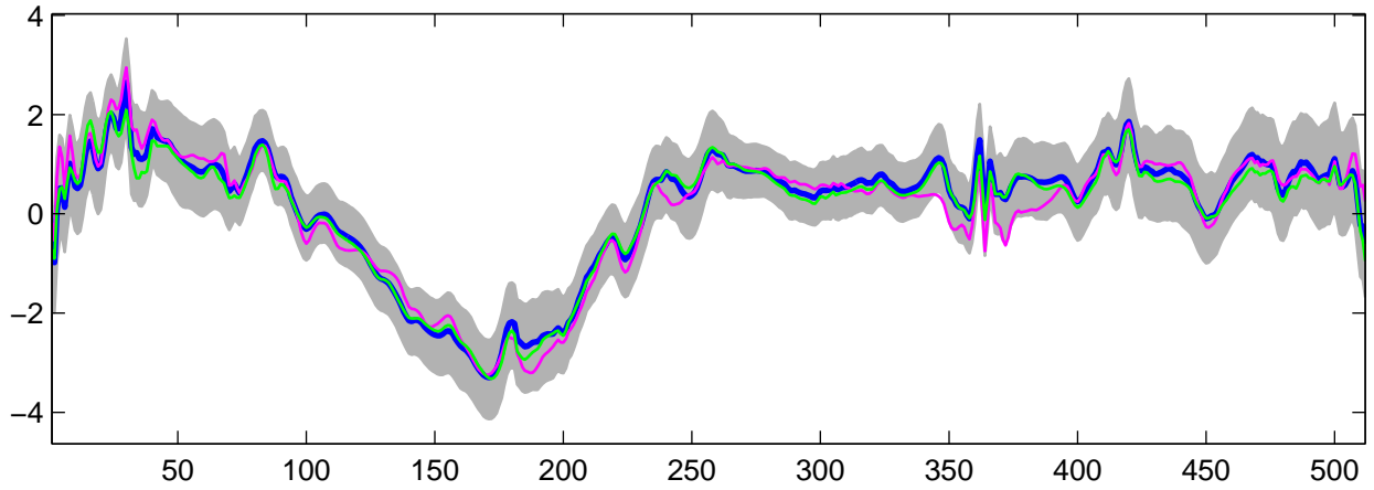
Estimated U_{12}(t) using G-WFMM: DE data, run 4
