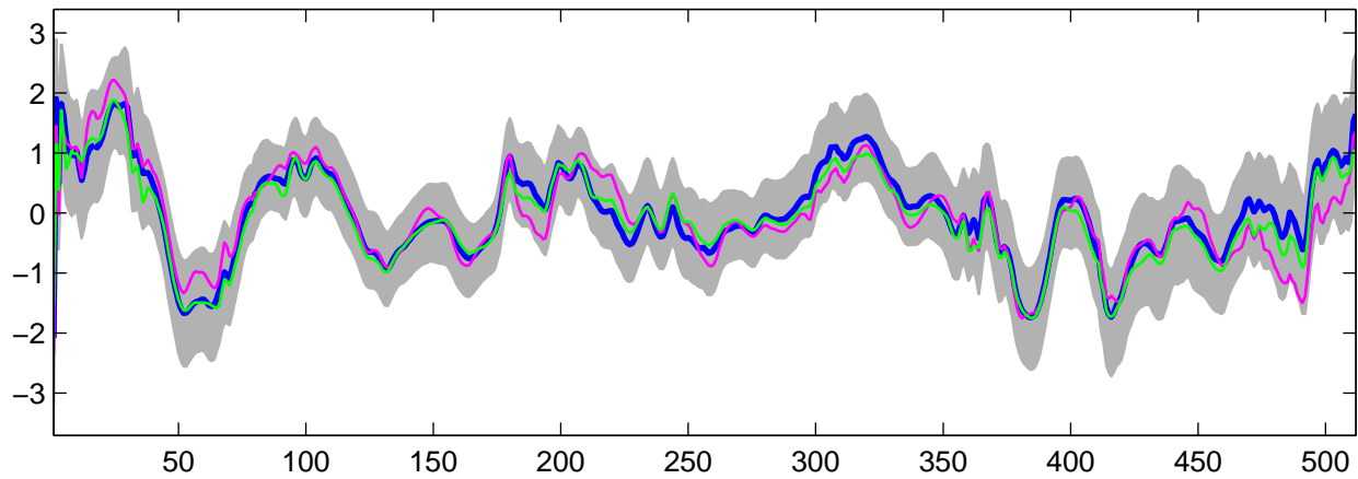
Estimated U_{12}(t) using G-WFMM: Normal data, run 4
