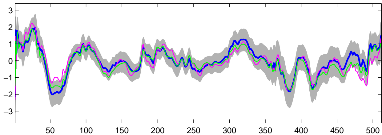
Estimated U_{12}(t) using R-WFMM: Normal data, run 4
