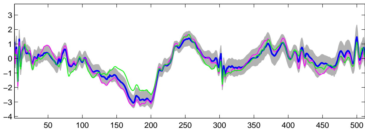
Estimated U_{12}(t) using R-WFMM: t_2 data, run 4
