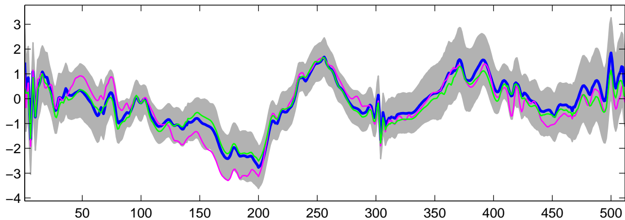
Estimated U_{12}(t) using G-WFMM: t_2 data, run 4
