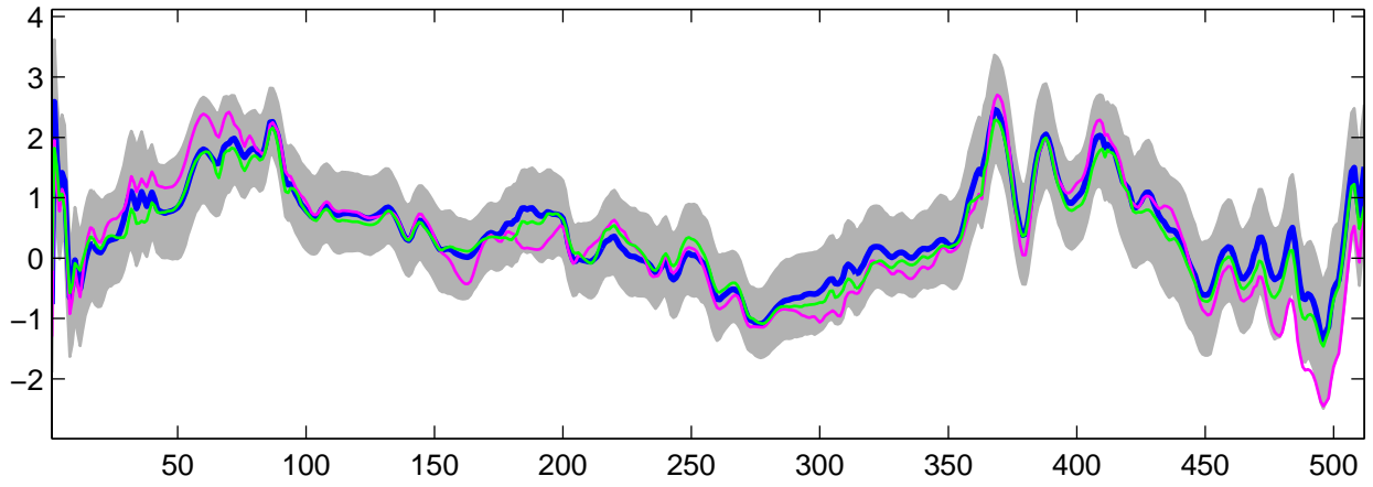
Estimated U_{13}(t) using G-WFMM: Normal data, run 4
