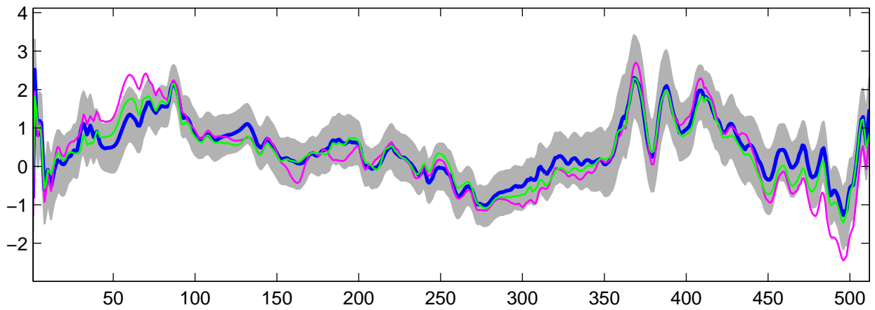
Estimated U_{13}(t) using R-WFMM: Normal data, run 4
