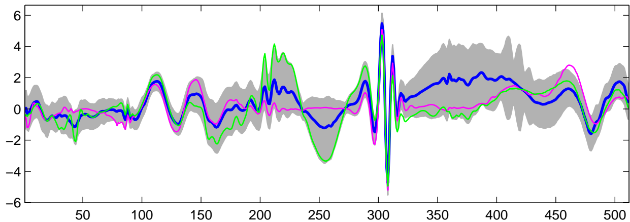
Estimated U_{13}(t) using G-WFMM: t_1 data, run 4
