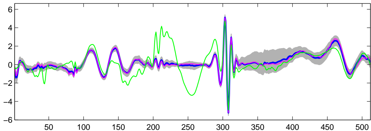
Estimated U_{13}(t) using R-WFMM: t_1 data, run 4
