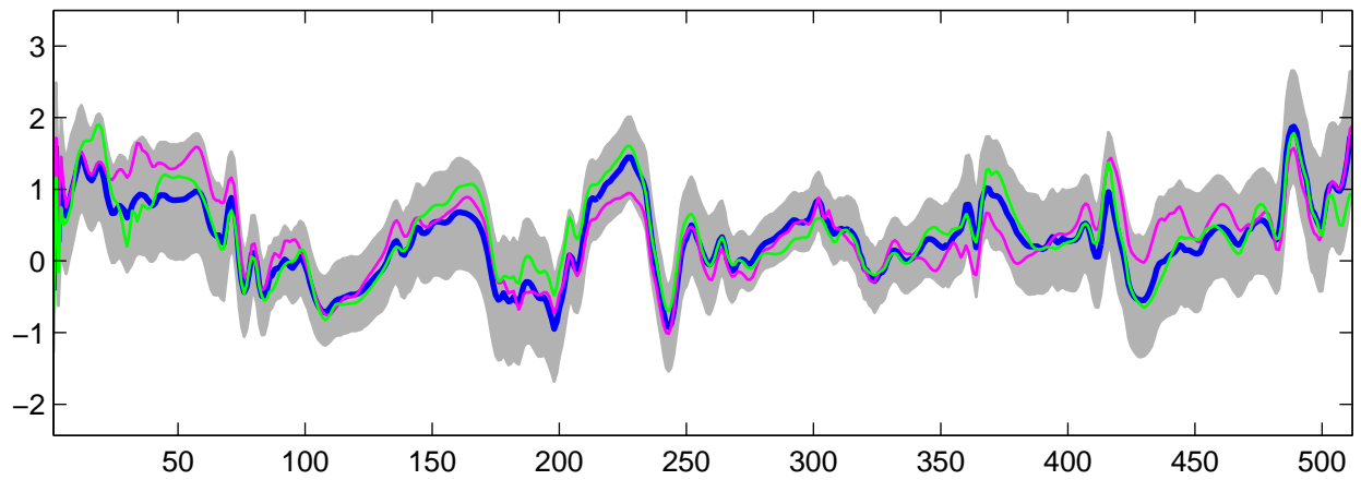
Estimated U_{14}(t) using R-WFMM: DE data, run 4
