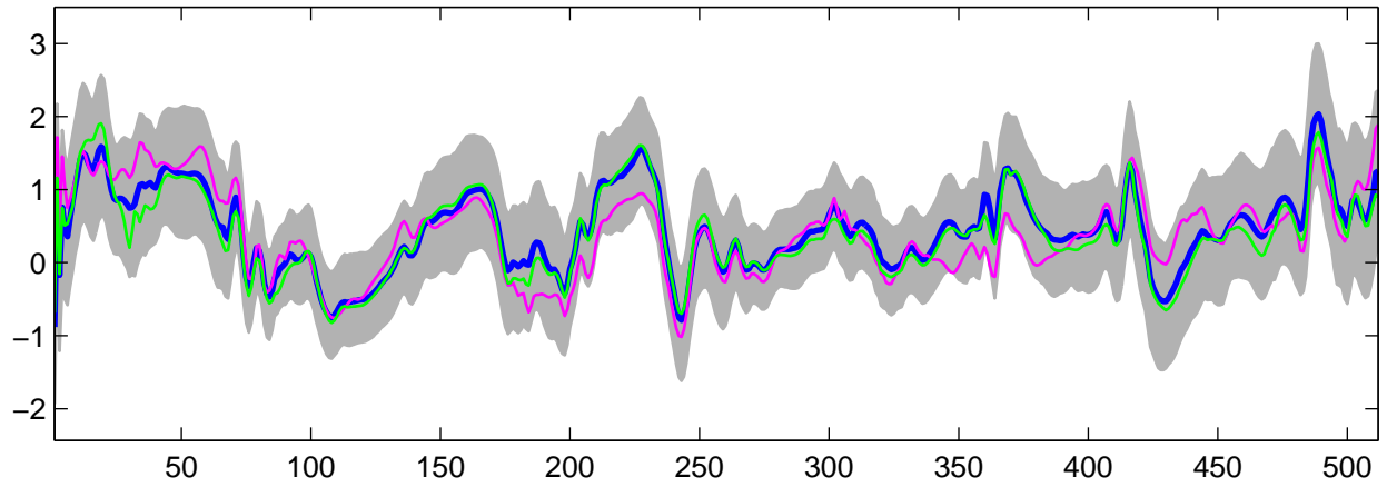
Estimated U_{14}(t) using G-WFMM: DE data, run 4
