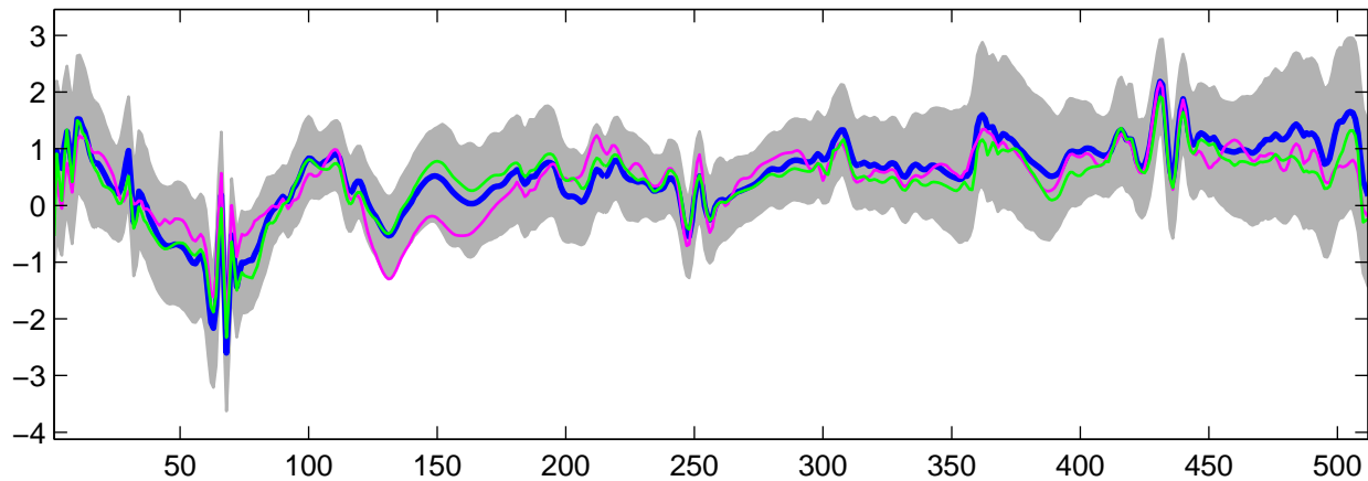
Estimated U_{14}(t) using G-WFMM: t_2 data, run 4
