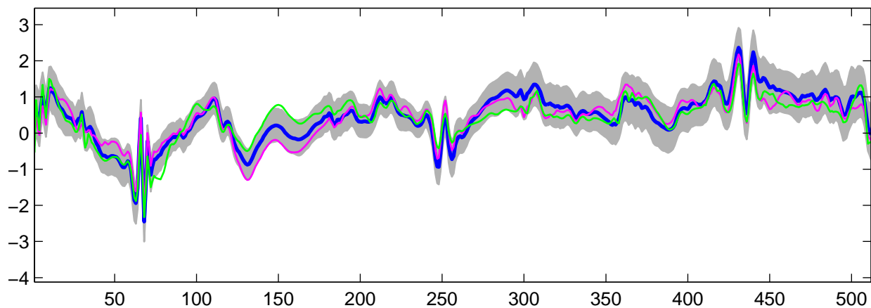
Estimated U_{14}(t) using R-WFMM: t_2 data, run 4
