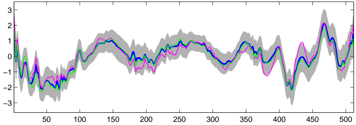
Estimated U_{15}(t) using G-WFMM: DE data, run 4
