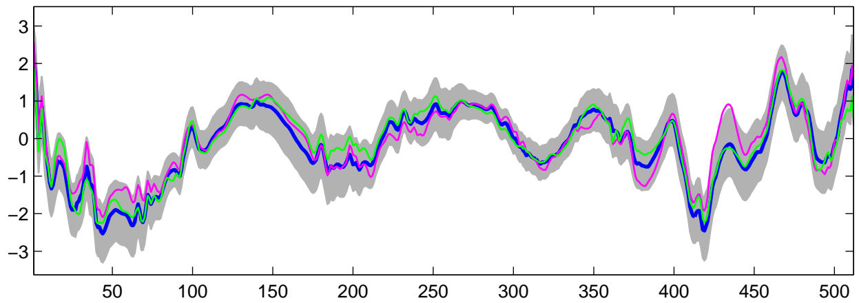
Estimated U_{15}(t) using R-WFMM: DE data, run 4
