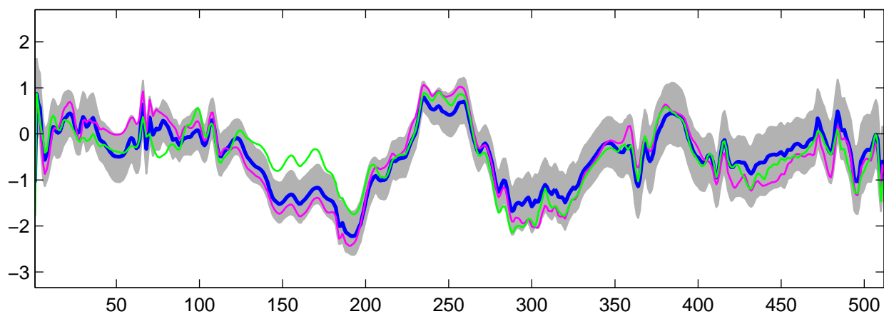
Estimated U_{15}(t) using R-WFMM: t_2 data, run 4
