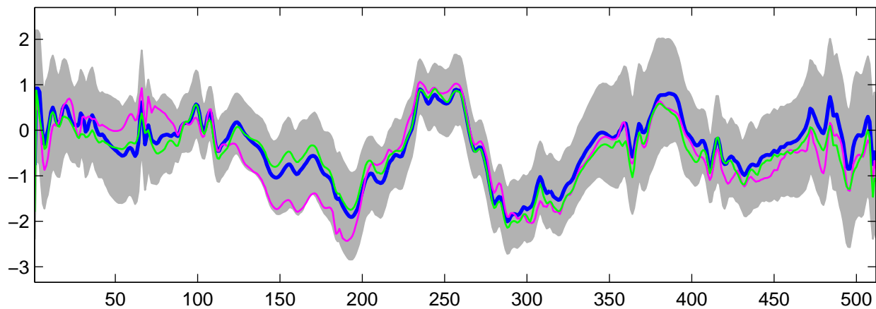
Estimated U_{15}(t) using G-WFMM: t_2 data, run 4
