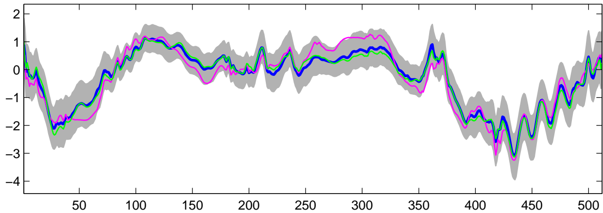
Estimated U_{15}(t) using G-WFMM: t_3 data, run 4
