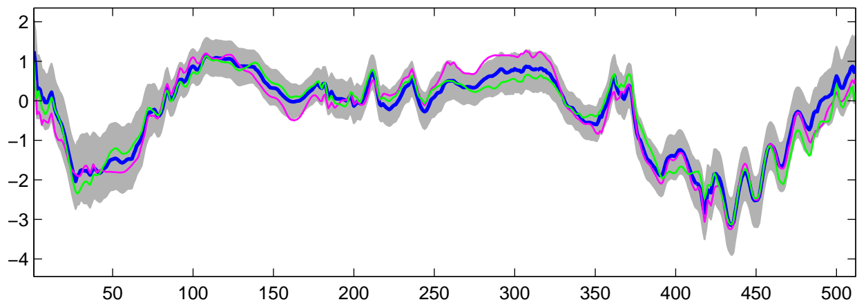
Estimated U_{15}(t) using R-WFMM: t_3 data, run 4
