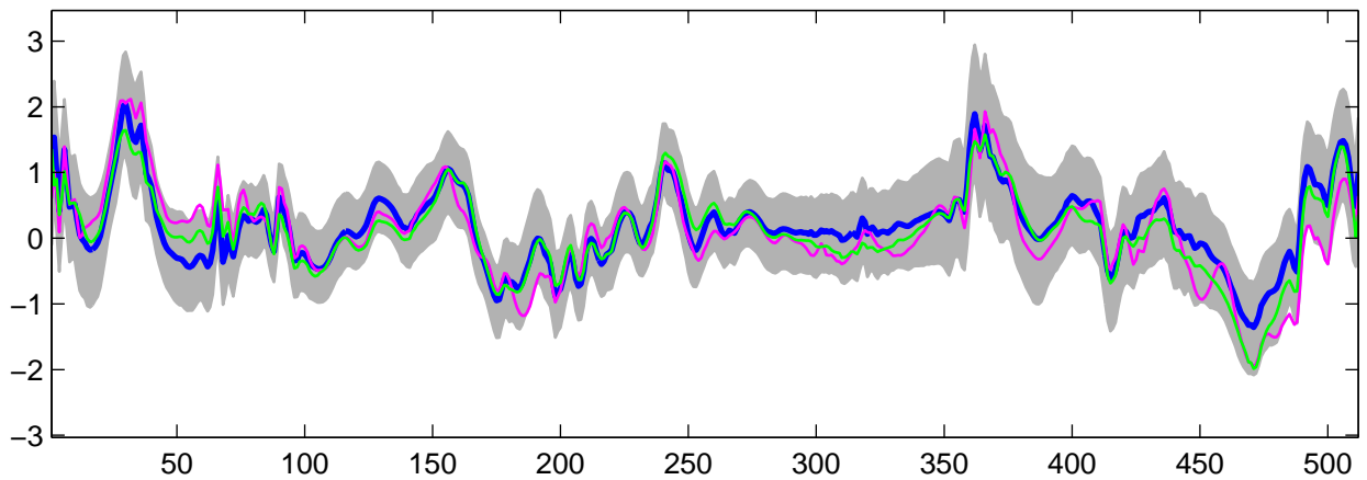
Estimated U_{16}(t) using R-WFMM: Normal data, run 4
