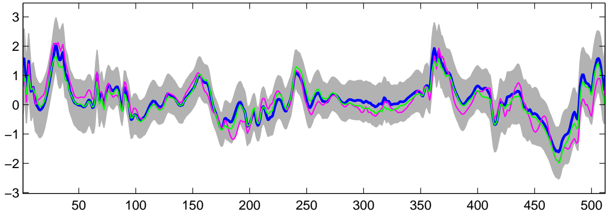
Estimated U_{16}(t) using G-WFMM: Normal data, run 4
