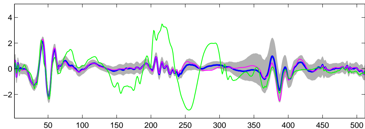
Estimated U_{16}(t) using R-WFMM: t_1 data, run 4
