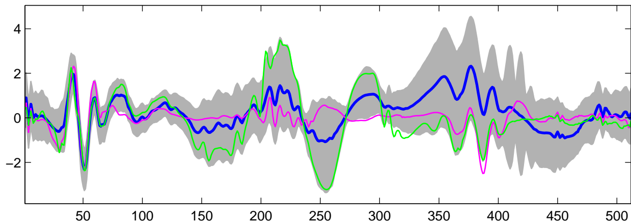
Estimated U_{16}(t) using G-WFMM: t_1 data, run 4
