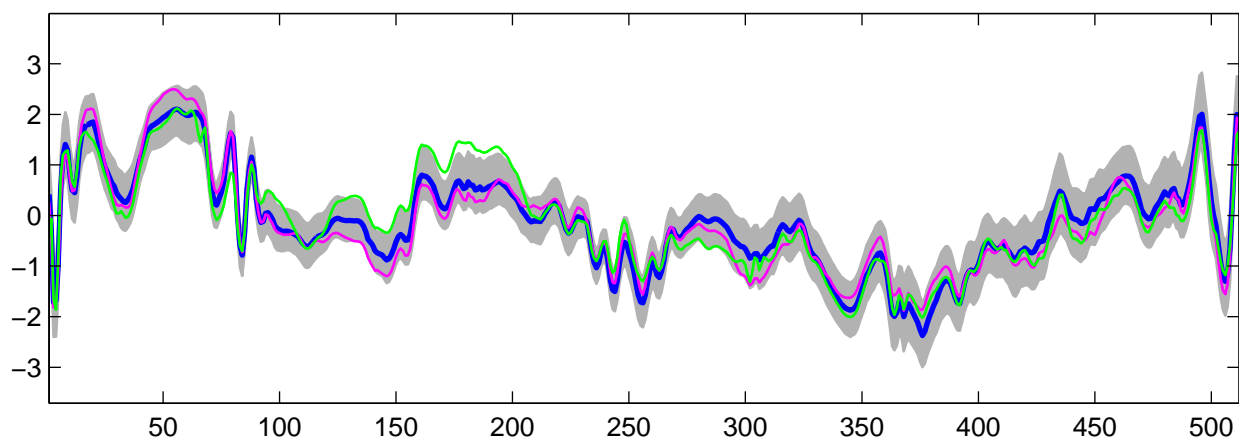
Estimated U_{16}(t) using R-WFMM: t_2 data, run 4
