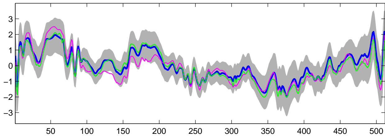
Estimated U_{16}(t) using G-WFMM: t_2 data, run 4
