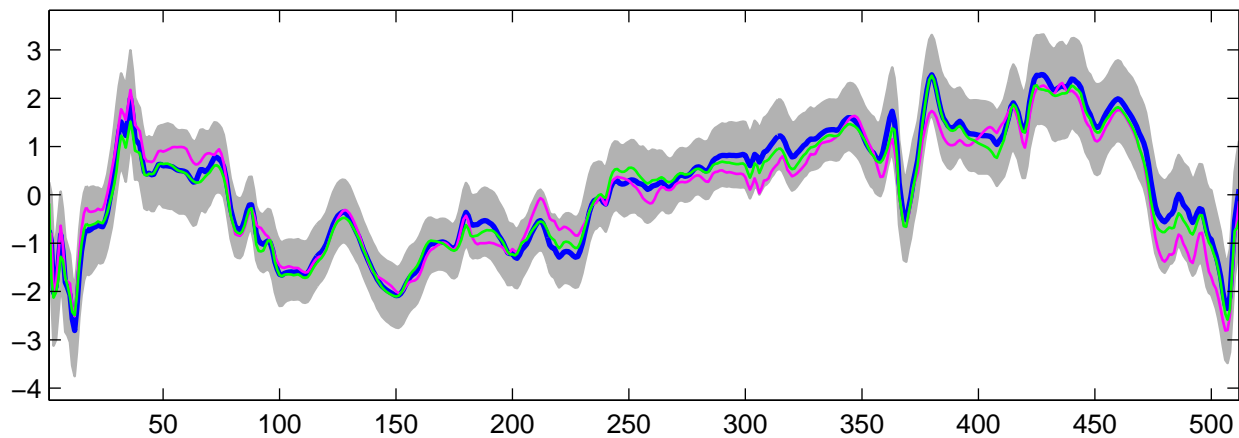
Estimated U_{17}(t) using G-WFMM: Normal data, run 4
