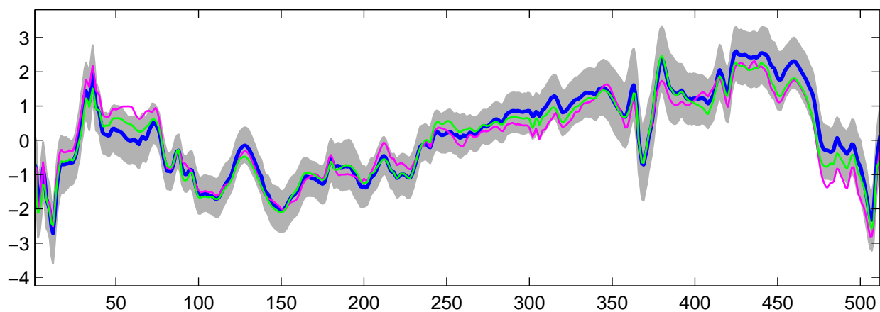
Estimated U_{17}(t) using R-WFMM: Normal data, run 4
