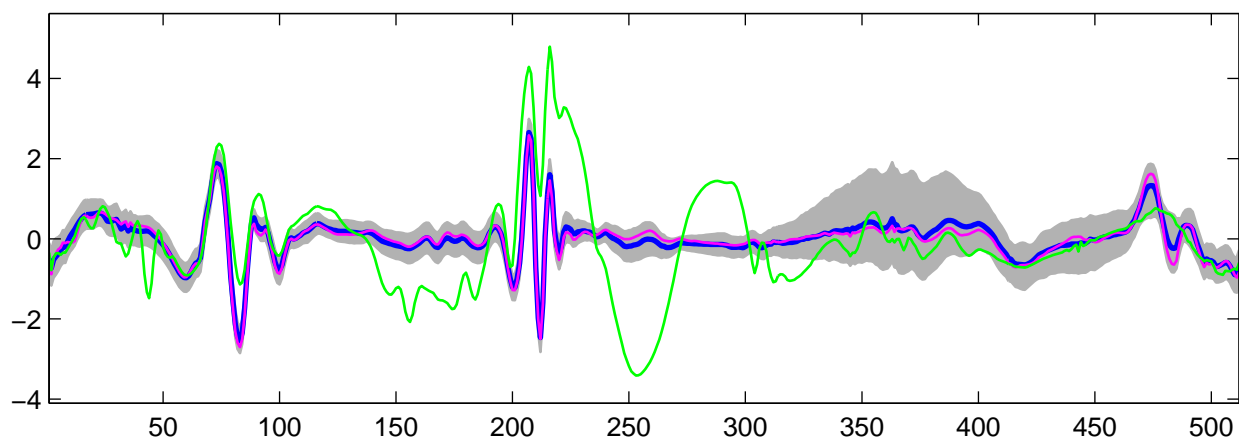
Estimated U_{17}(t) using R-WFMM: t_1 data, run 4
