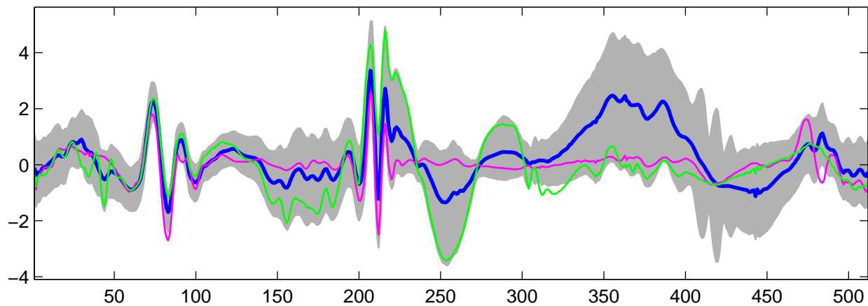
Estimated U_{17}(t) using G-WFMM: t_1 data, run 4
