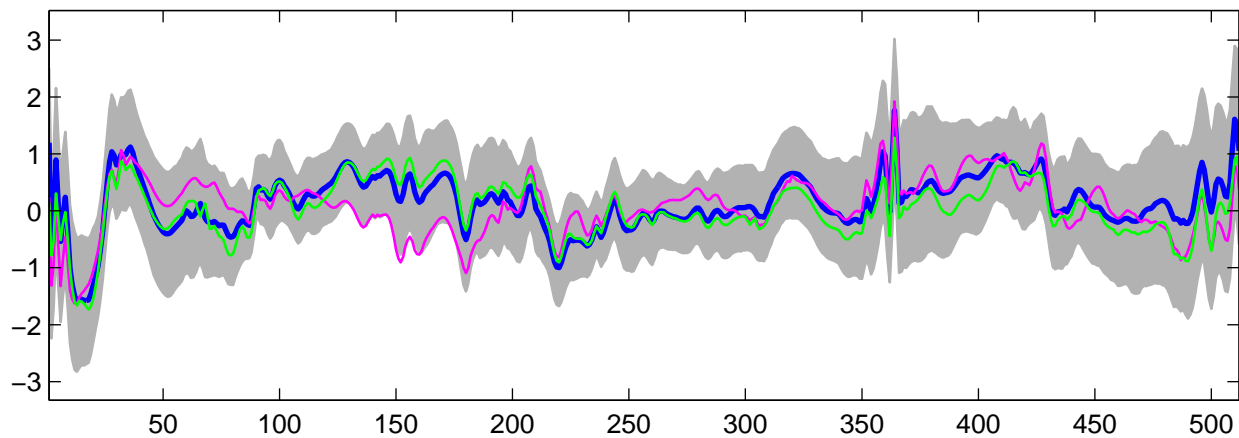
Estimated U_{17}(t) using G-WFMM: t_2 data, run 4
