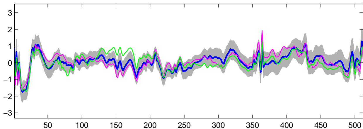
Estimated U_{17}(t) using R-WFMM: t_2 data, run 4
