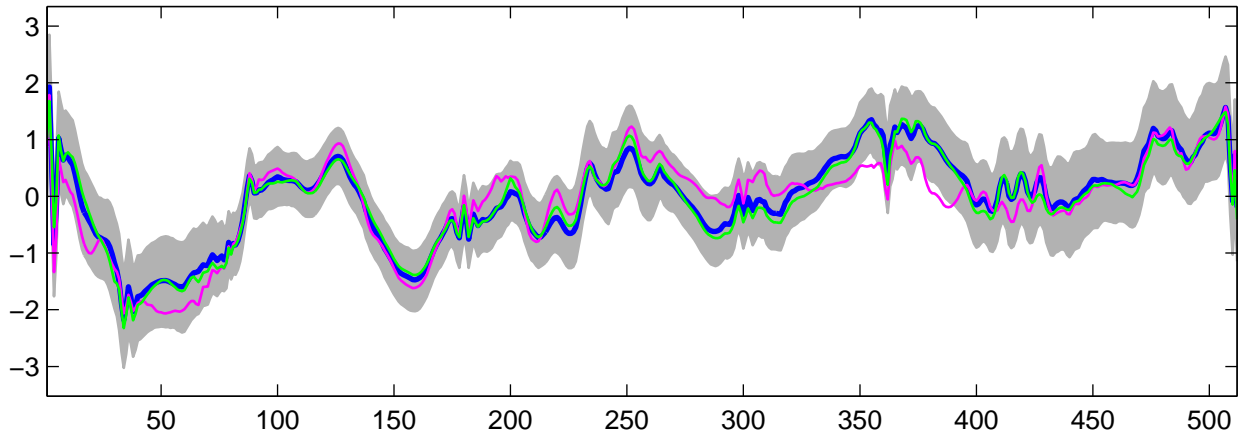
Estimated U_{17}(t) using G-WFMM: t_3 data, run 4
