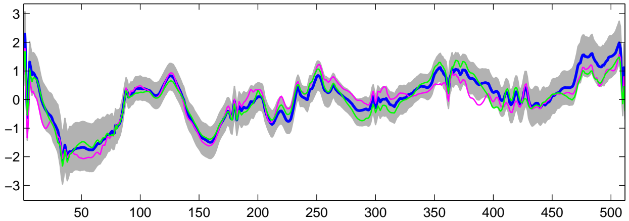
Estimated U_{17}(t) using R-WFMM: t_3 data, run 4
