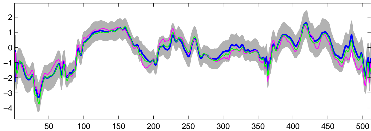
Estimated U_{18}(t) using G-WFMM: Normal data, run 4
