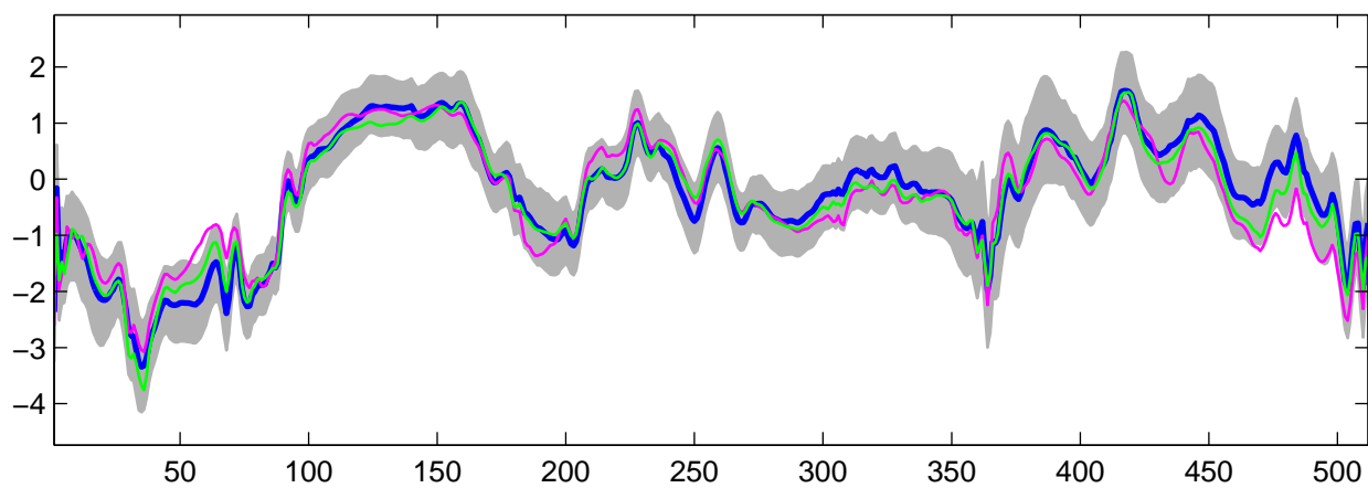
Estimated U_{18}(t) using R-WFMM: Normal data, run 4
