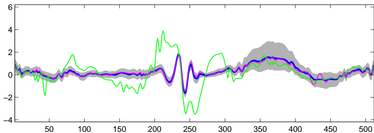
Estimated U_{18}(t) using R-WFMM: t_1 data, run 4
