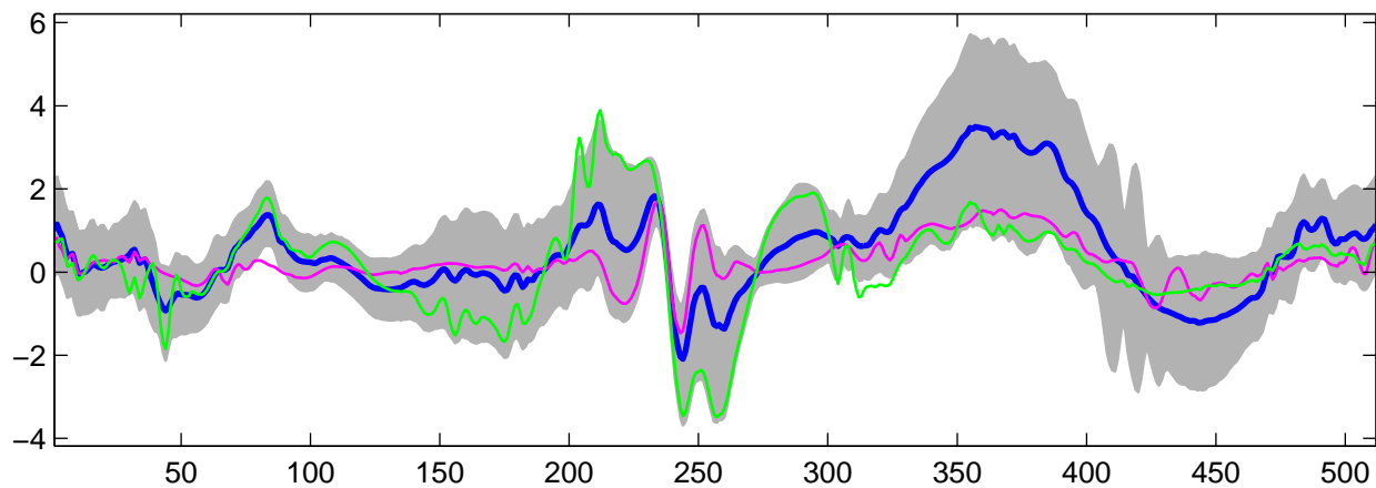
Estimated U_{18}(t) using G-WFMM: t_1 data, run 4
