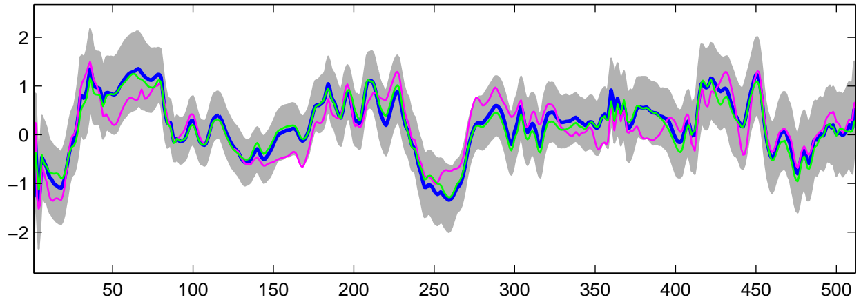
Estimated U_{18}(t) using G-WFMM: t_3 data, run 4
