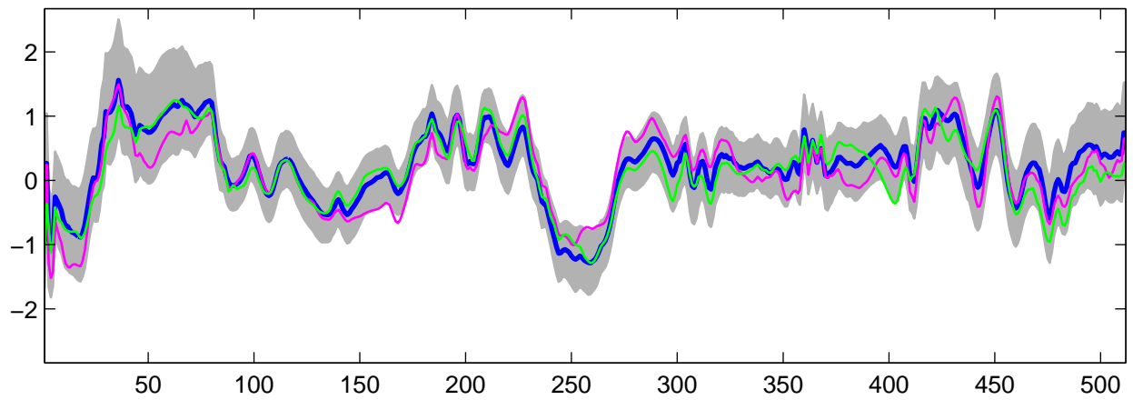
Estimated U_{18}(t) using R-WFMM: t_3 data, run 4
