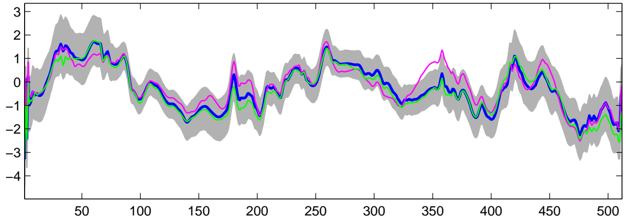
Estimated U_{19}(t) using G-WFMM: DE data, run 4
