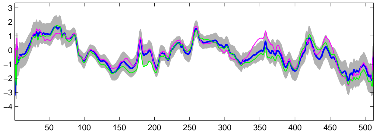
Estimated U_{19}(t) using R-WFMM: DE data, run 4
