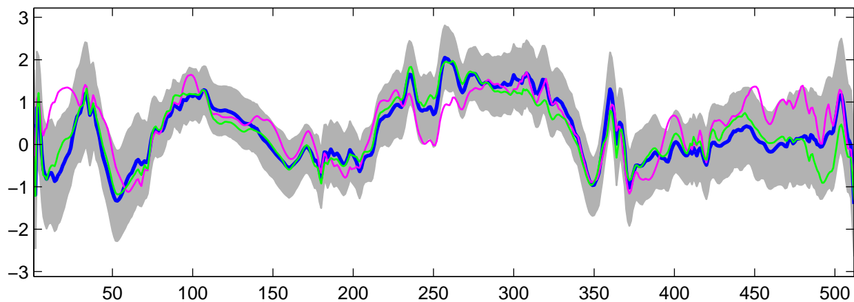
Estimated U_{19}(t) using R-WFMM: Normal data, run 4
