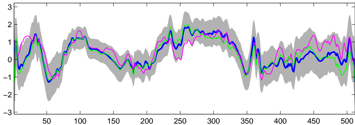
Estimated U_{19}(t) using G-WFMM: Normal data, run 4
