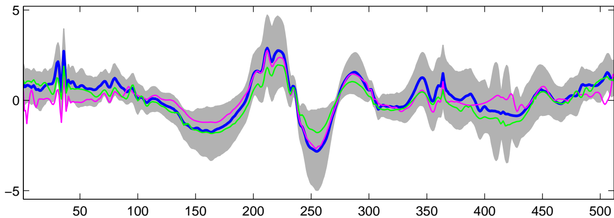
Estimated U_{19}(t) using G-WFMM: t_1 data, run 4
