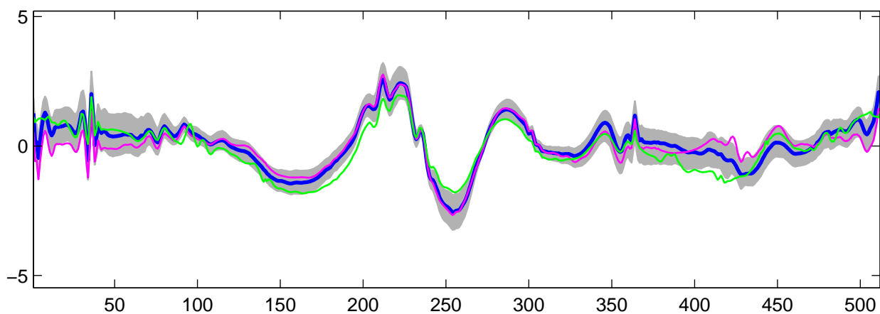
Estimated U_{19}(t) using R-WFMM: t_1 data, run 4
