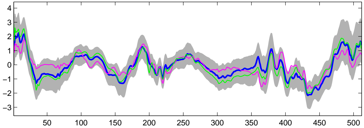
Estimated U_{19}(t) using G-WFMM: t_2 data, run 4
