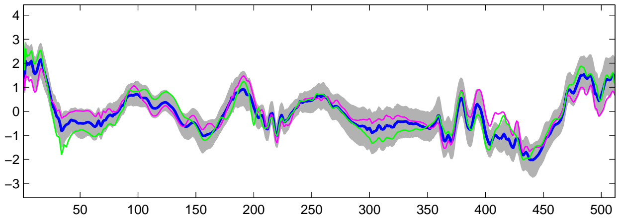
Estimated U_{19}(t) using R-WFMM: t_2 data, run 4
