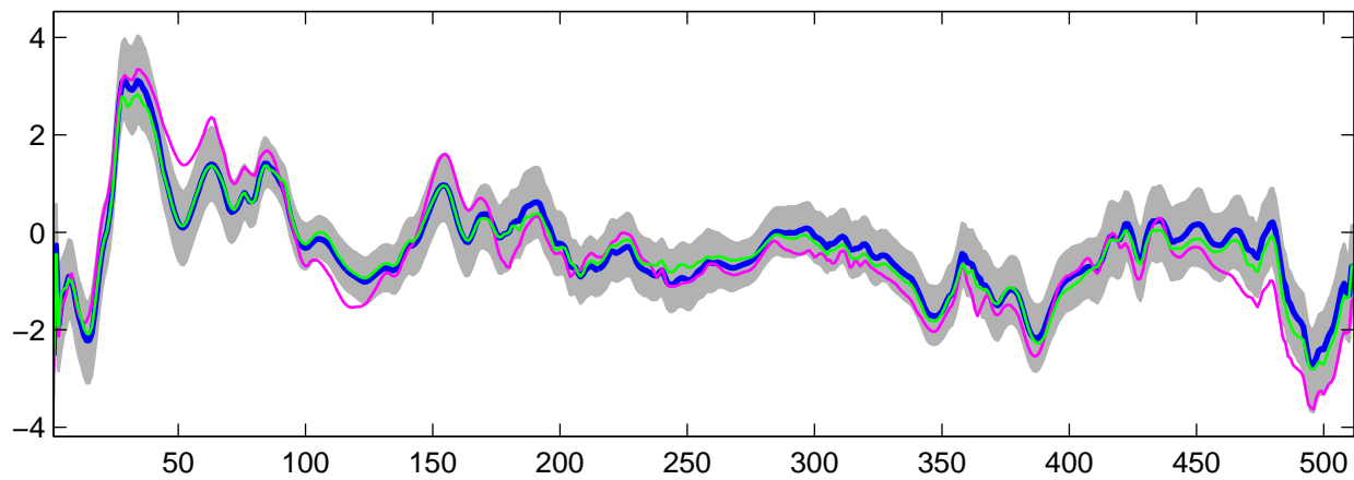
Estimated U_1(t) using G-WFMM: DE data, run 4
