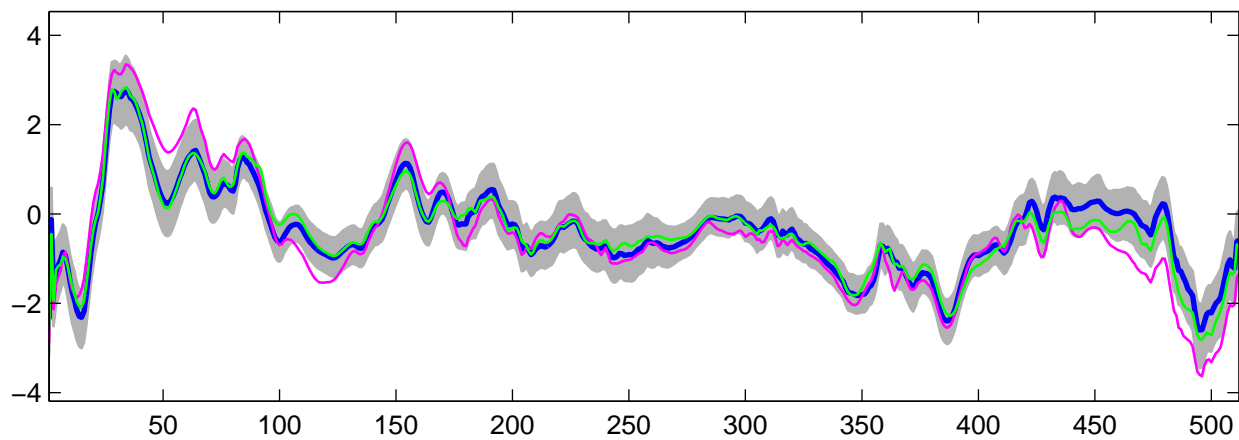
Estimated U_1(t) using R-WFMM: DE data, run 4
