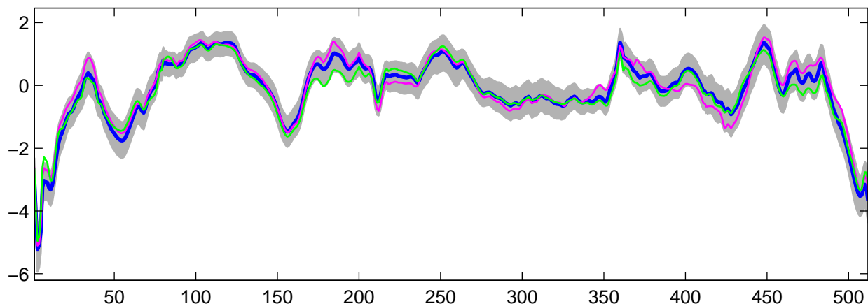
Estimated U_1(t) using R-WFMM: t_3 data, run 4
