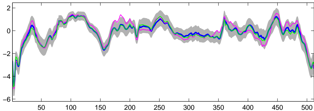
Estimated U_1(t) using G-WFMM: t_3 data, run 4
