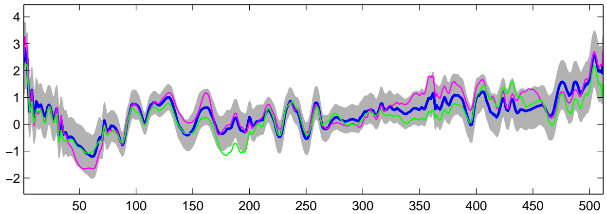
Estimated U_{20}(t) using R-WFMM: DE data, run 4
