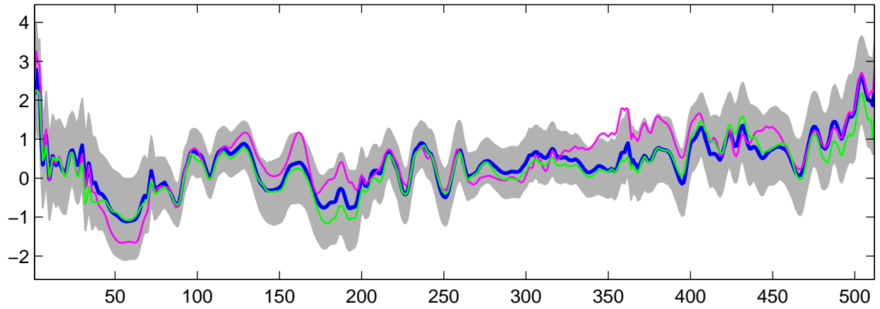
Estimated U_{20}(t) using G-WFMM: DE data, run 4
