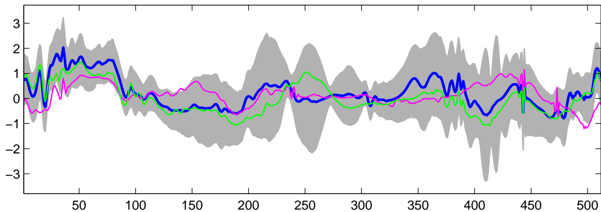
Estimated U_{20}(t) using G-WFMM: t_1 data, run 4
