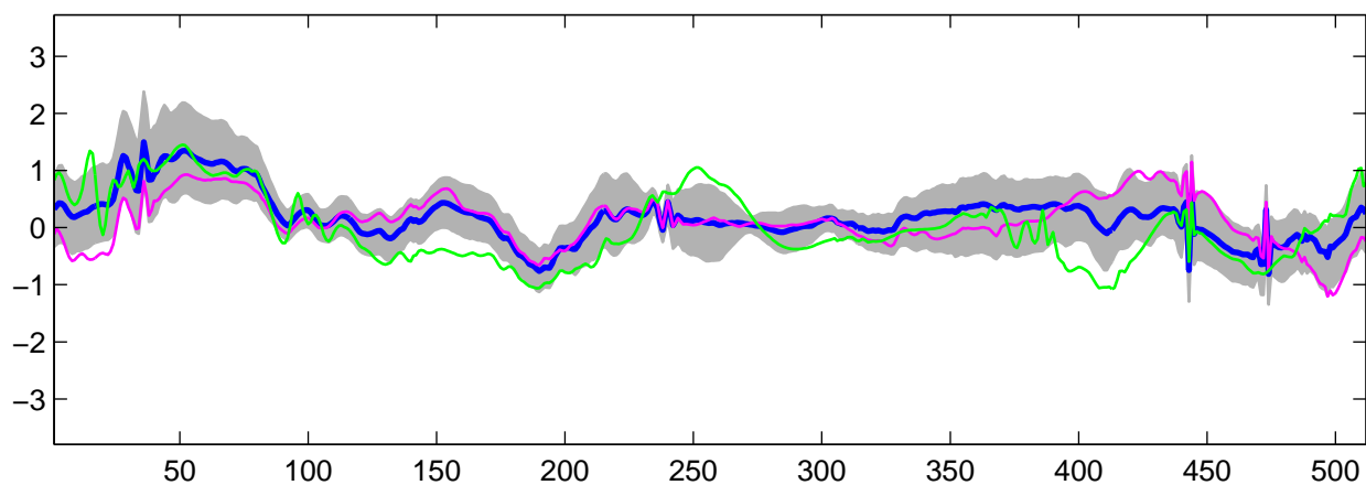
Estimated U_{20}(t) using R-WFMM: t_1 data, run 4
