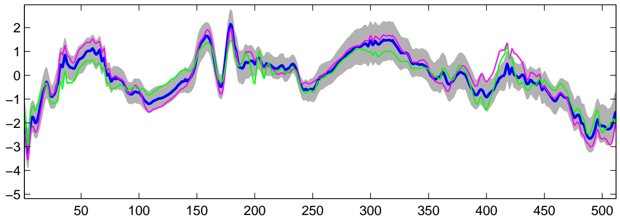
Estimated U_{20}(t) using R-WFMM: t_2 data, run 4
