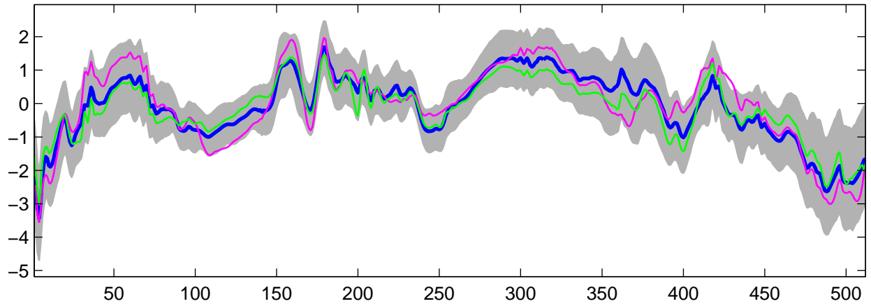
Estimated U_{20}(t) using G-WFMM: t_2 data, run 4
