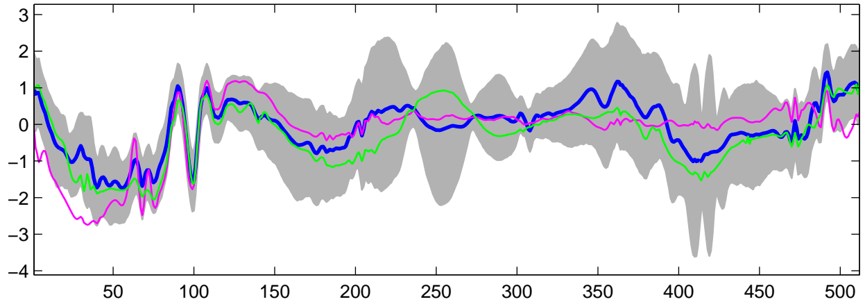
Estimated U_{21}(t) using G-WFMM: t_1 data, run 4
