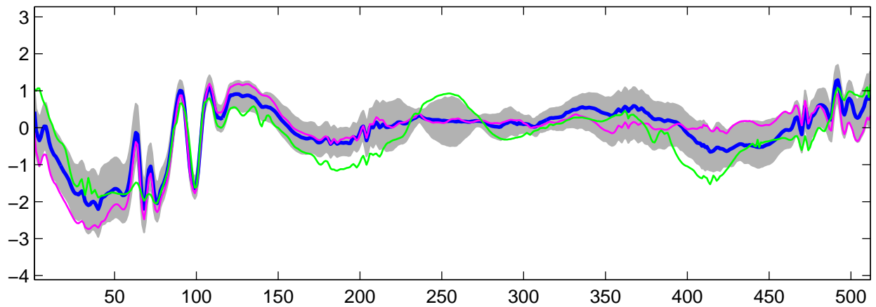
Estimated U_{21}(t) using R-WFMM: t_1 data, run 4
