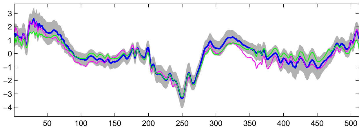
Estimated U_{21}(t) using R-WFMM: t_3 data, run 4
