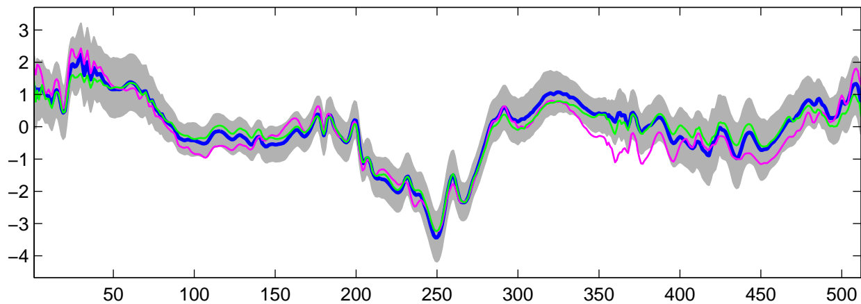
Estimated U_{21}(t) using G-WFMM: t_3 data, run 4
