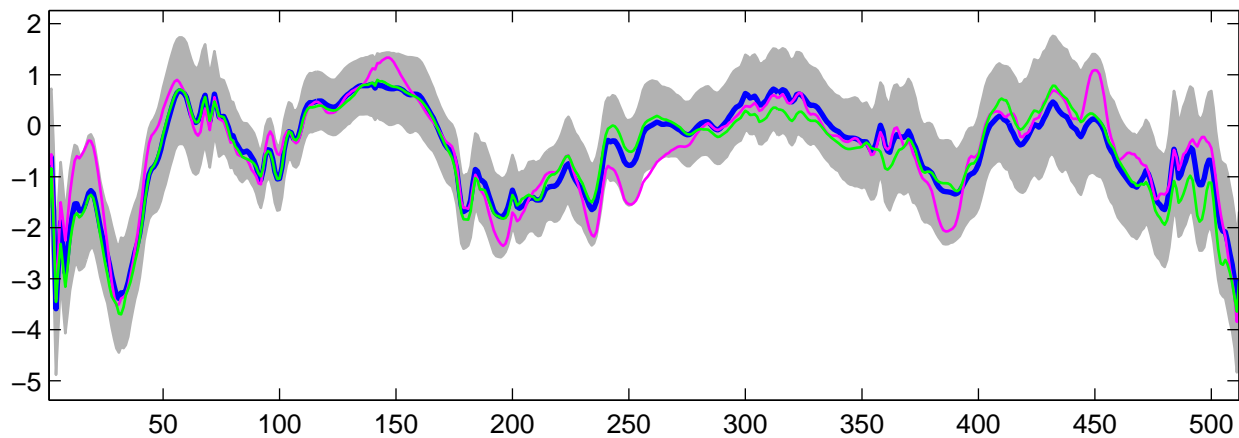
Estimated U_{22}(t) using G-WFMM: Normal data, run 4
