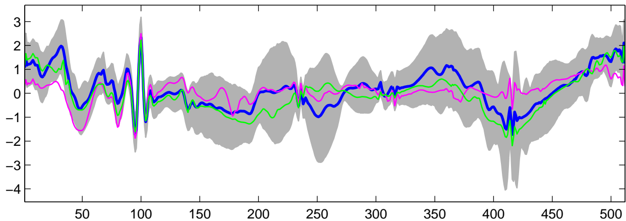
Estimated U_{22}(t) using G-WFMM: t_1 data, run 4
