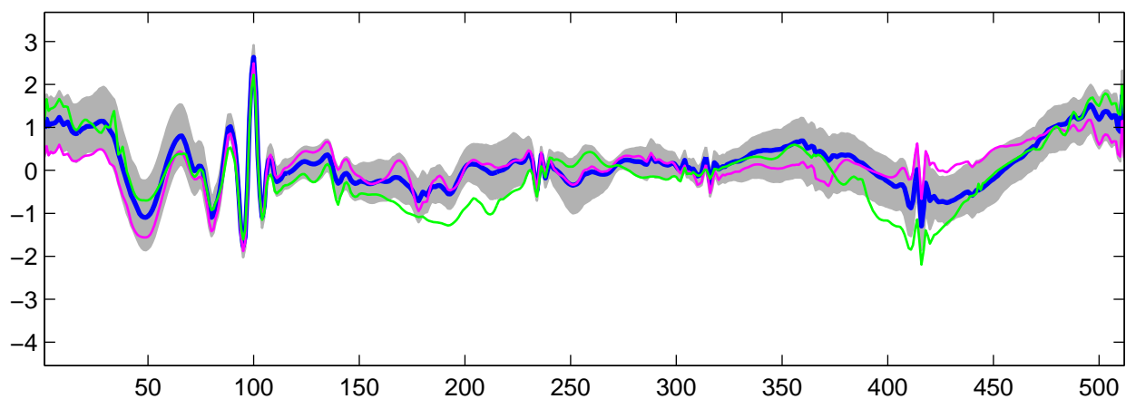
Estimated U_{22}(t) using R-WFMM: t_1 data, run 4
