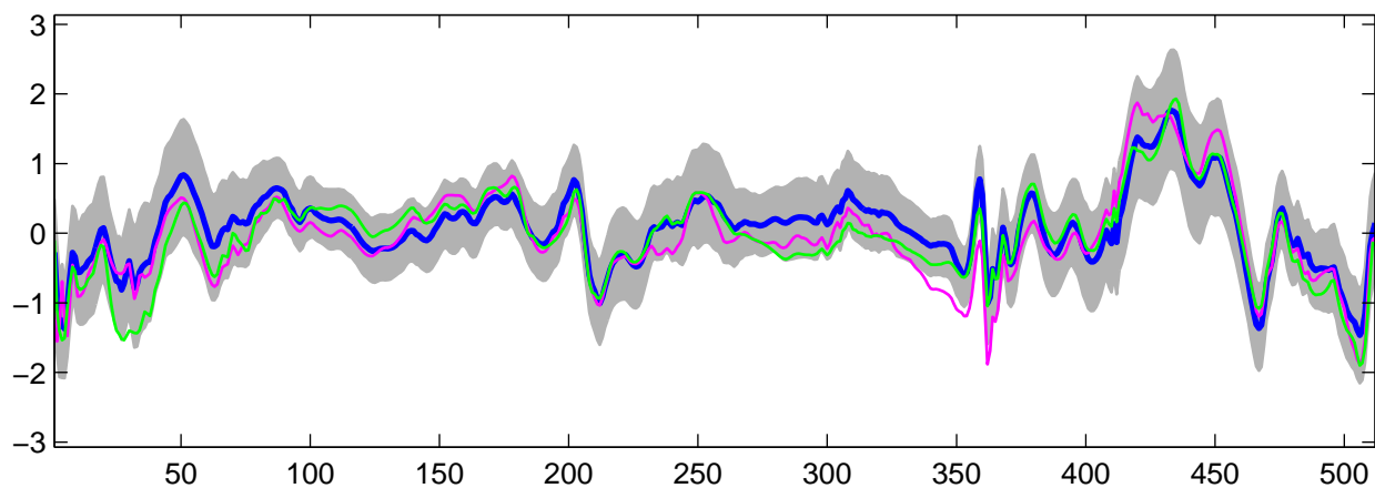
Estimated U_{22}(t) using R-WFMM: t_3 data, run 4
