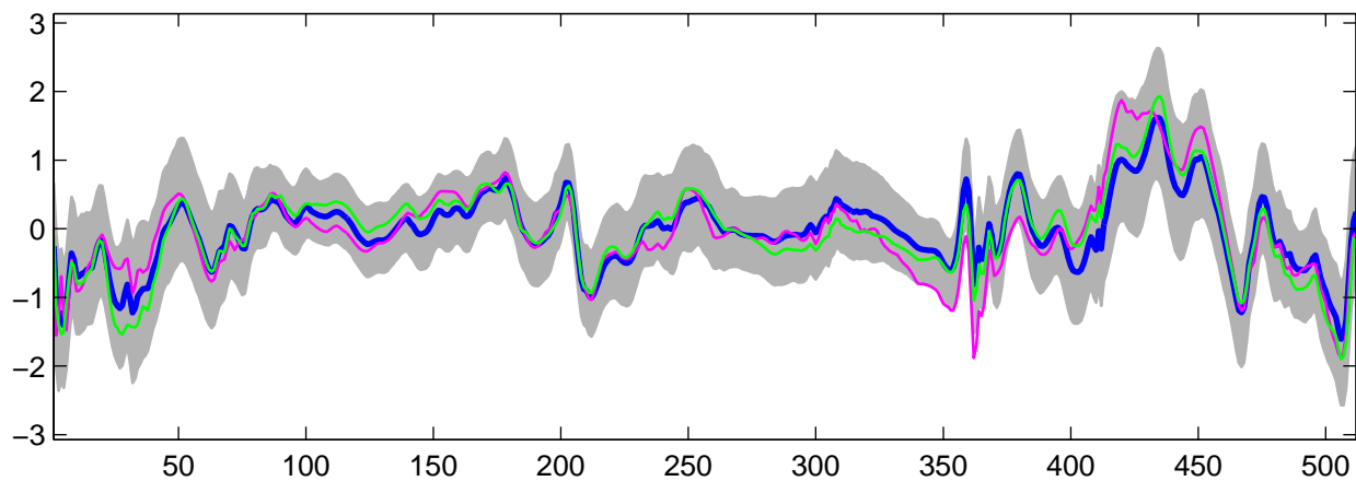
Estimated U_{22}(t) using G-WFMM: t_3 data, run 4
