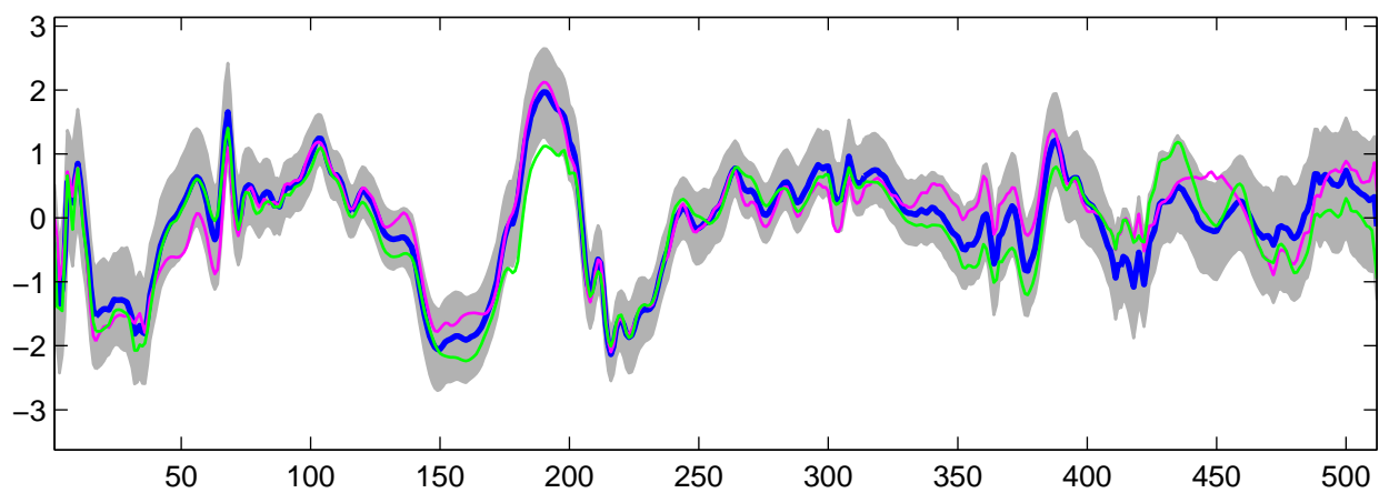
Estimated U_{23}(t) using R-WFMM: DE data, run 4
