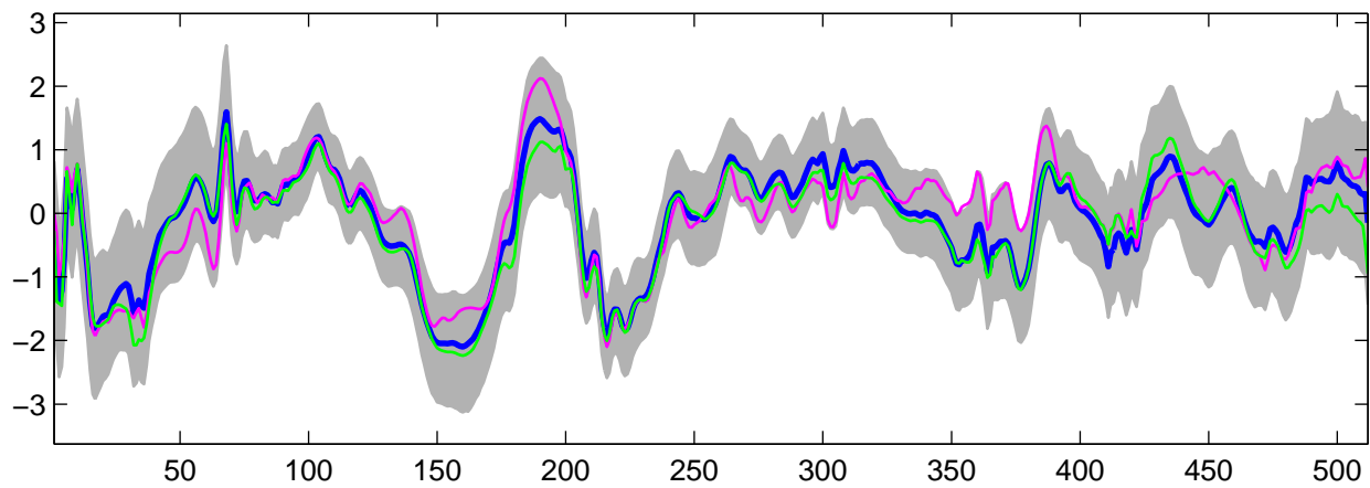
Estimated U_{23}(t) using G-WFMM: DE data, run 4
