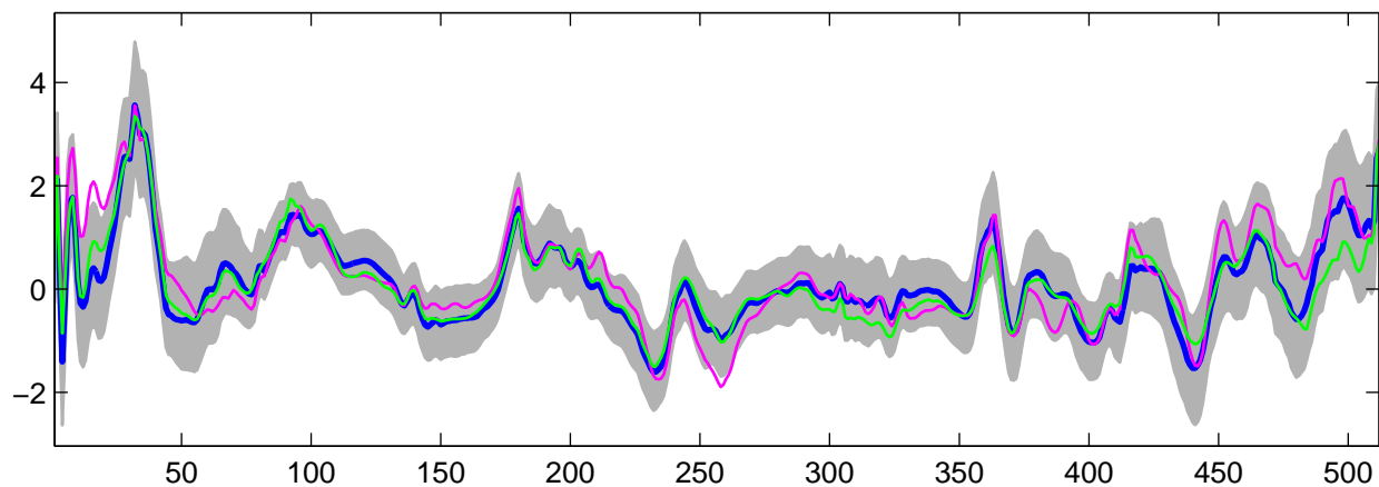
Estimated U_{23}(t) using R-WFMM: Normal data, run 4
