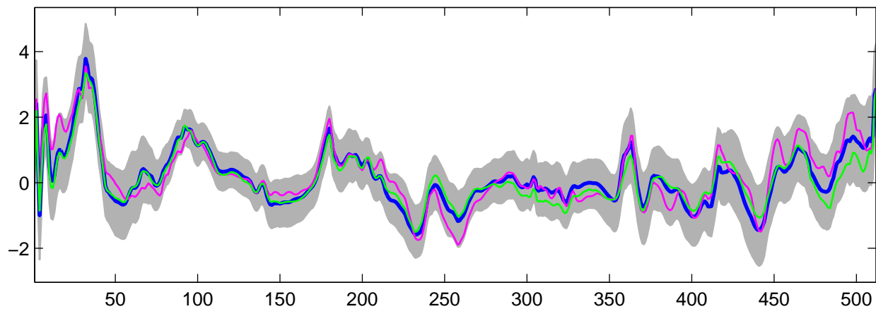
Estimated U_{23}(t) using G-WFMM: Normal data, run 4
