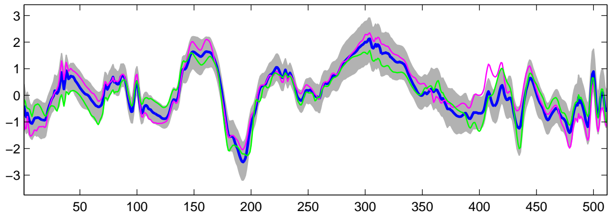
Estimated U_{23}(t) using R-WFMM: t_2 data, run 4
