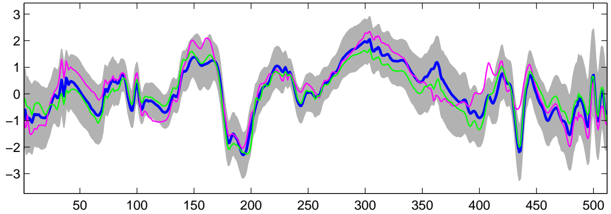
Estimated U_{23}(t) using G-WFMM: t_2 data, run 4
