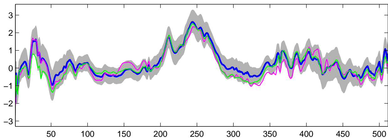
Estimated U_{23}(t) using R-WFMM: t_3 data, run 4
