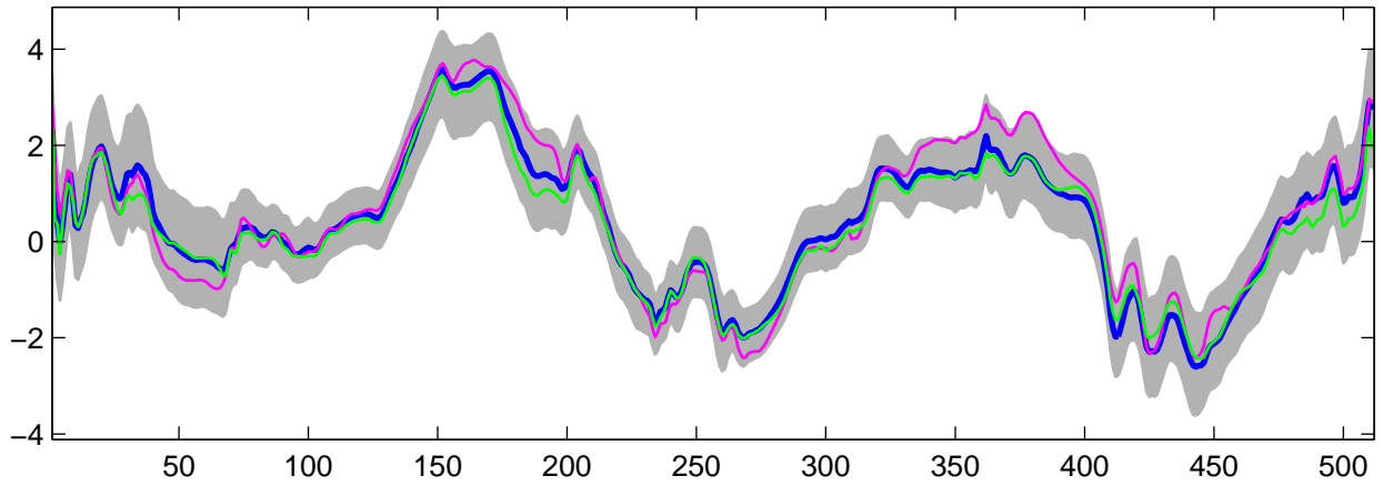
Estimated U_{24}(t) using G-WFMM: DE data, run 4
