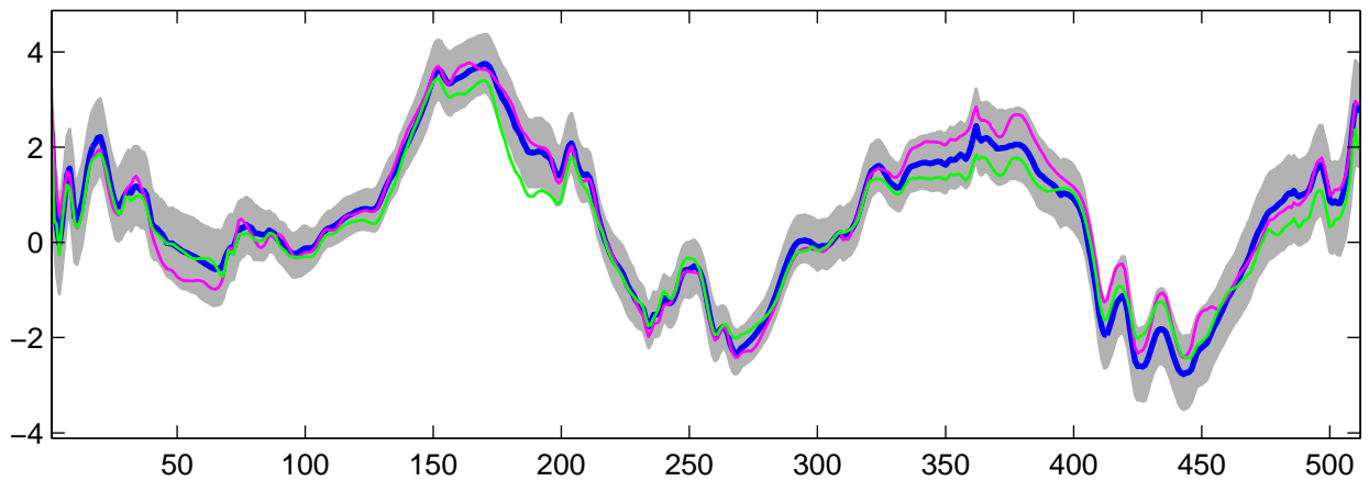
Estimated U_{24}(t) using R-WFMM: DE data, run 4
