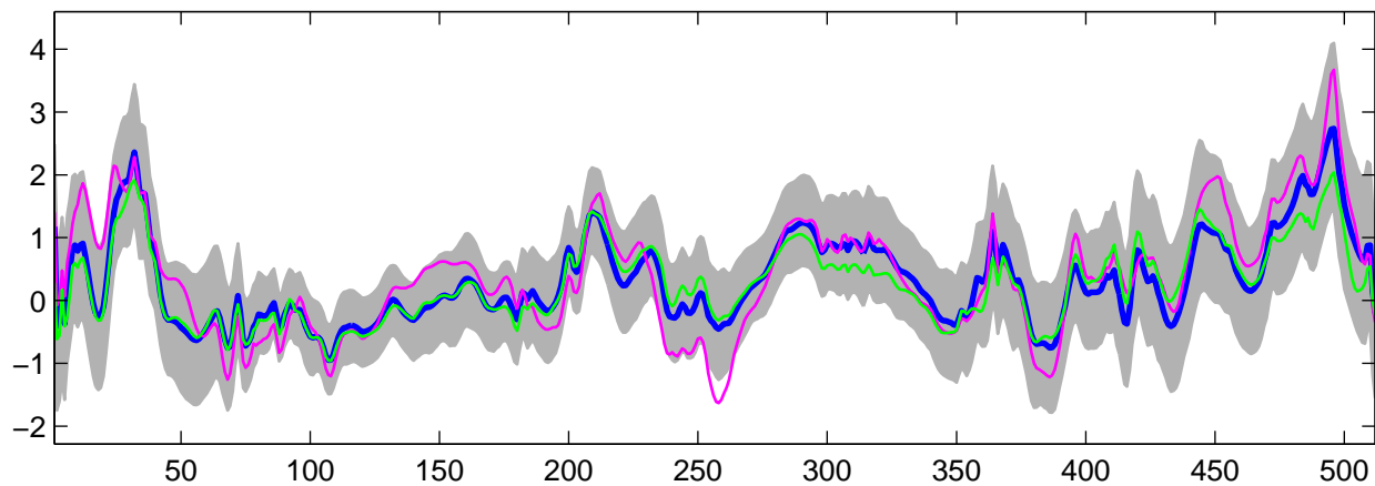
Estimated U_{24}(t) using G-WFMM: Normal data, run 4
