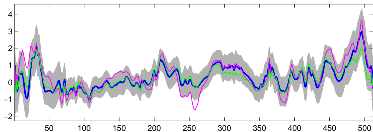
Estimated U_{24}(t) using R-WFMM: Normal data, run 4
