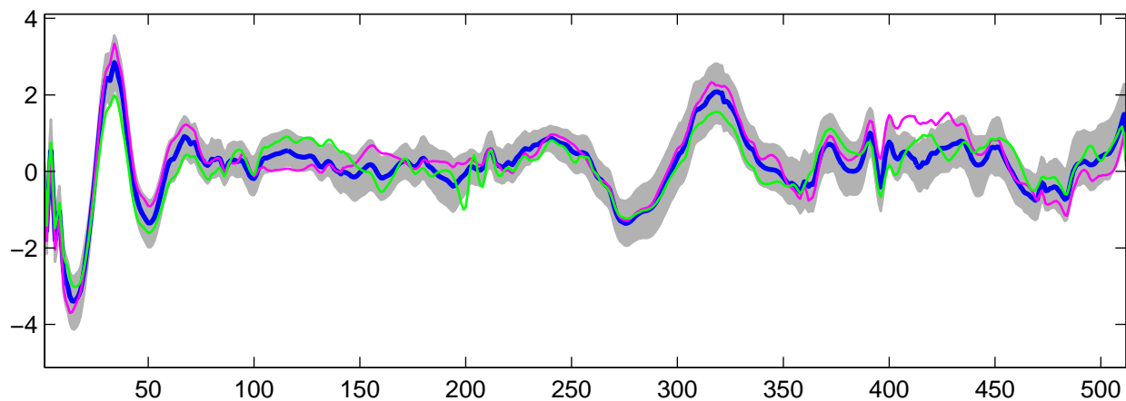
Estimated U_{24}(t) using R-WFMM: t_2 data, run 4
