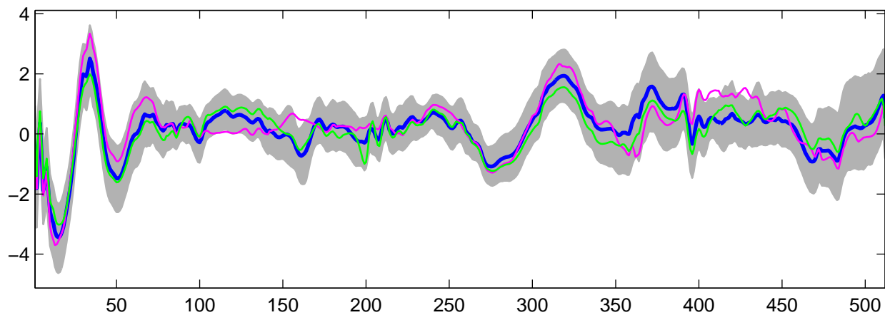
Estimated U_{24}(t) using G-WFMM: t_2 data, run 4
