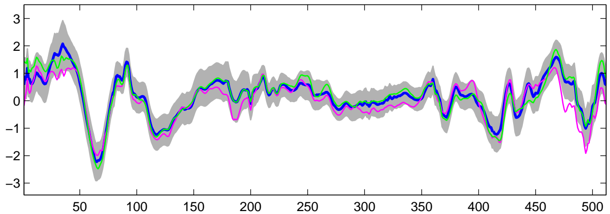
Estimated U_{25}(t) using R-WFMM: DE data, run 4
