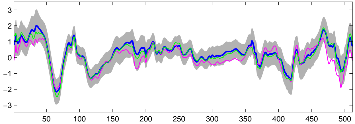
Estimated U_{25}(t) using G-WFMM: DE data, run 4
