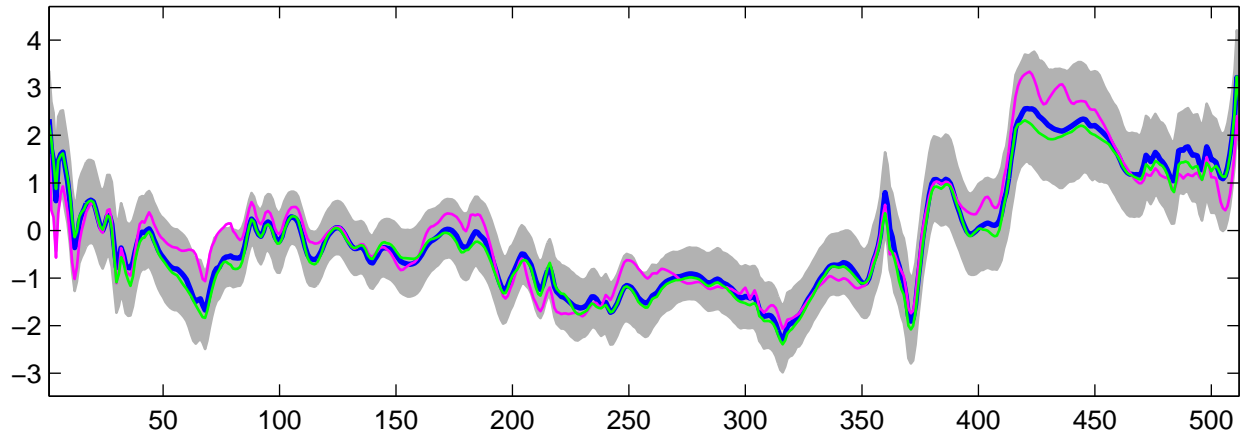
Estimated U_{25}(t) using G-WFMM: Normal data, run 4
