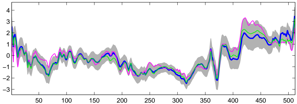
Estimated U_{25}(t) using R-WFMM: Normal data, run 4
