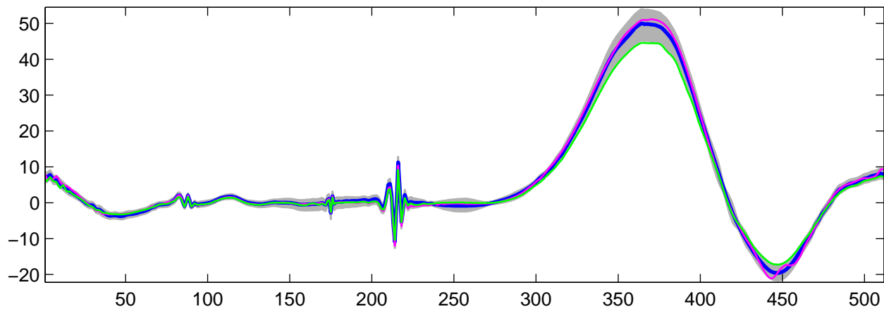
Estimated U_{25}(t) using G-WFMM: t_1 data, run 4
