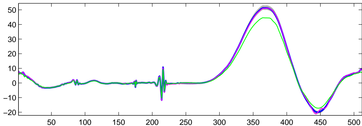
Estimated U_{25}(t) using R-WFMM: t_1 data, run 4
