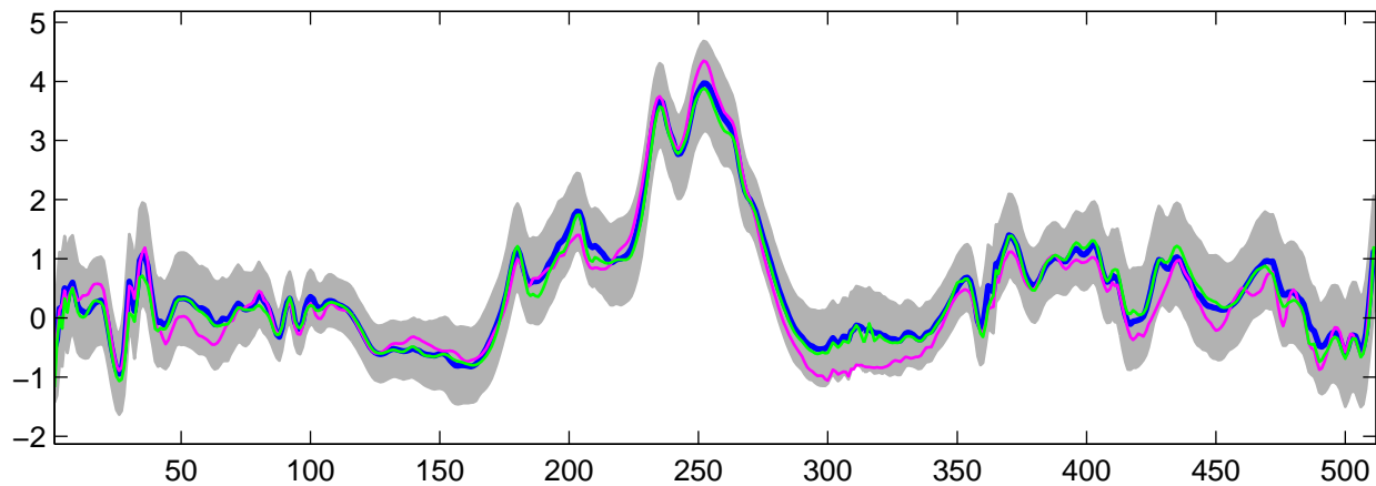
Estimated U_{25}(t) using G-WFMM: t_3 data, run 4
