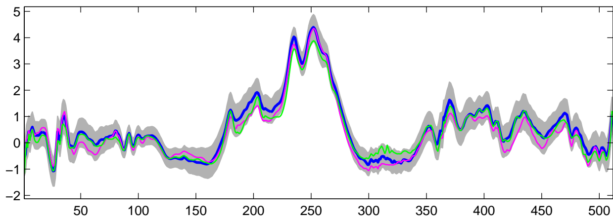
Estimated U_{25}(t) using R-WFMM: t_3 data, run 4
