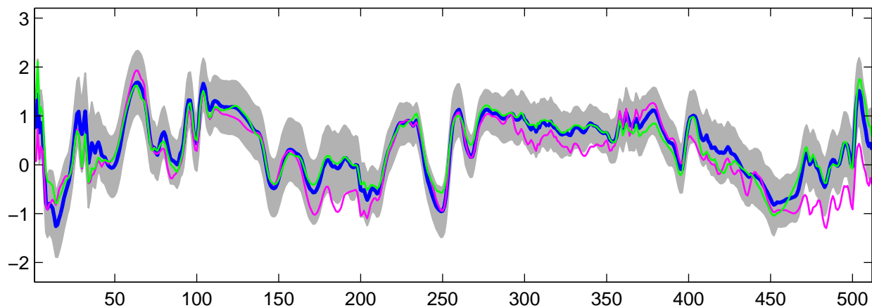
Estimated U_{26}(t) using R-WFMM: DE data, run 4
