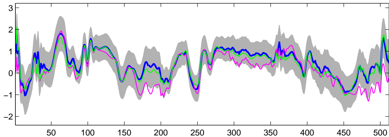
Estimated U_{26}(t) using G-WFMM: DE data, run 4
