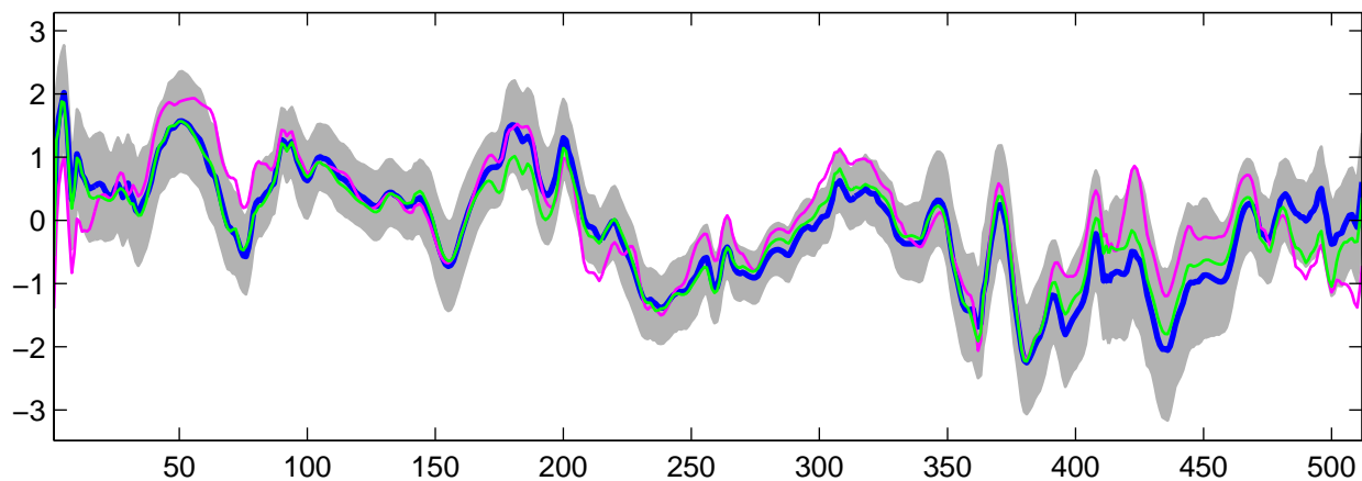
Estimated U_{26}(t) using R-WFMM: Normal data, run 4
