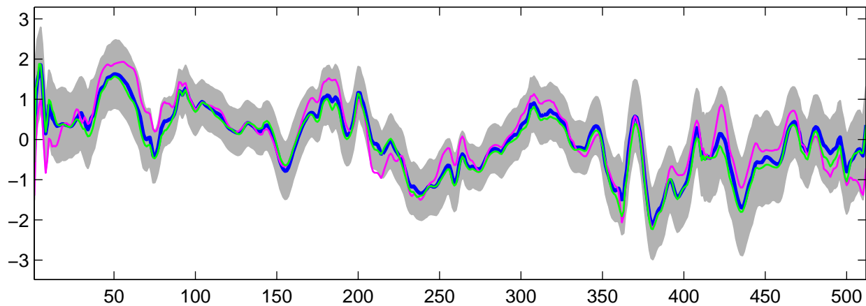
Estimated U_{26}(t) using G-WFMM: Normal data, run 4
