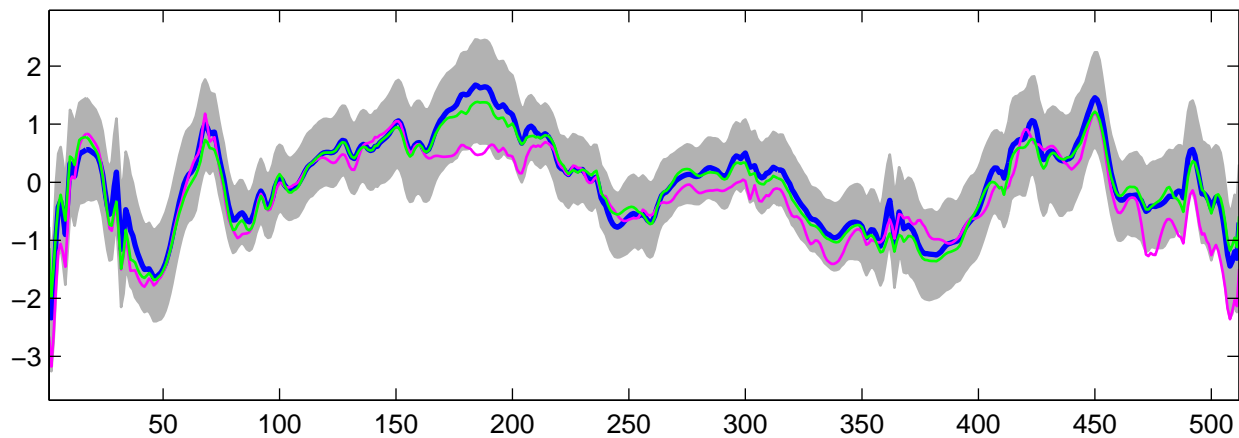
Estimated U_{27}(t) using G-WFMM: DE data, run 4
