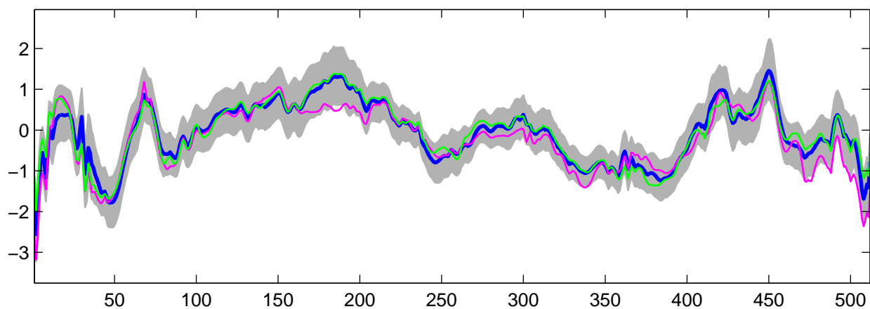
Estimated U_{27}(t) using R-WFMM: DE data, run 4
