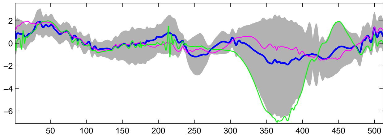
Estimated U_{27}(t) using G-WFMM: t_1 data, run 4
