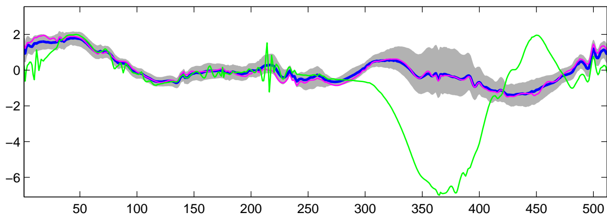
Estimated U_{27}(t) using R-WFMM: t_1 data, run 4
